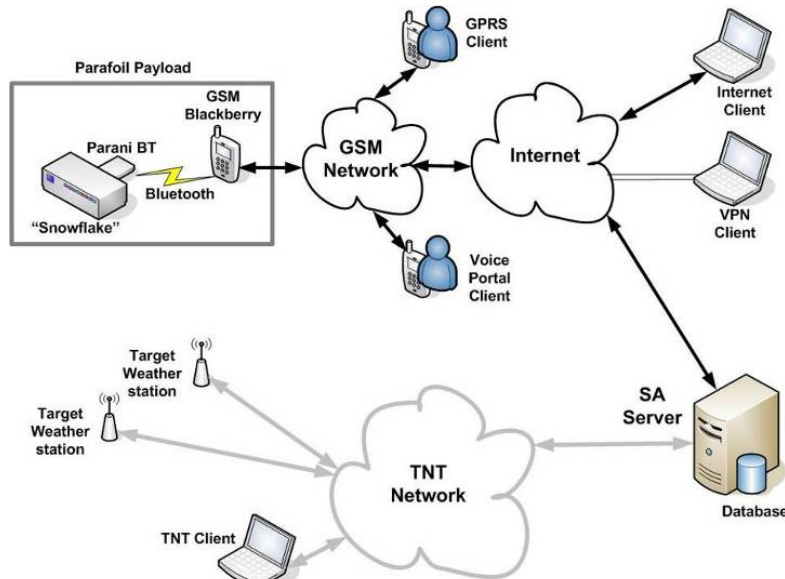
Fig. 6 Communication block diagram.
