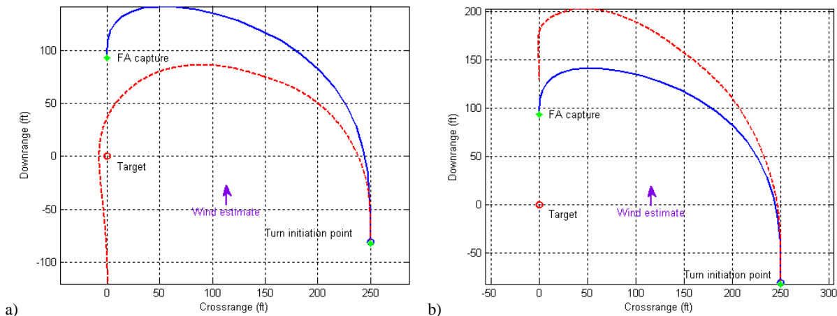
Fig. 1 Optimal guidance with constant unaccounted 5ft/s winds: “extra” head wind (a) and “extra” tail wind (b).
