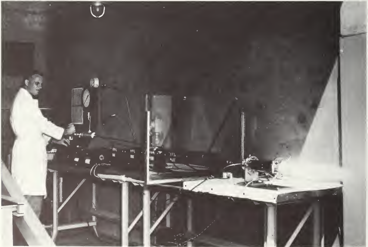
A candidate for the Aeronautical Engineer Degree performing experiments at one of the rocket test cells.
