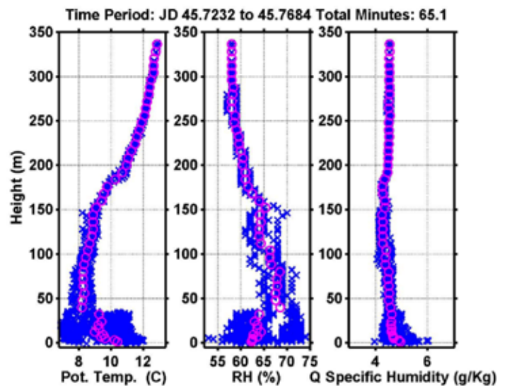
Figure 1. Meteorological data from a radiosonde using InstantEye as a measurement platform. Plots (left to right) show (1) potential temperature, (2) relative humidity and (3) specific humidity. Blue crosses show individual data points while purple circles are elevation-binned median values. The large variability below 50 m is due to the atmospheric warming up over the course of the hour of the experiment. Only two profiles went above this level and only one above 150 m, therefore less variability is seen at the higher elevations. Note the bend in the data around 150 m; this indicates the level where the surface solar heating effect had reached at the time of the measurements. Also note the average (purple circle) decrease in temperature and specific humidity right above the surface indicating upward fluxes of sensible heat and moisture (latent heat). This is what was expected for these conditions and demonstrates the usefulness of this system for these very low locations that are not well-resolved with standard weather balloon measurements.
